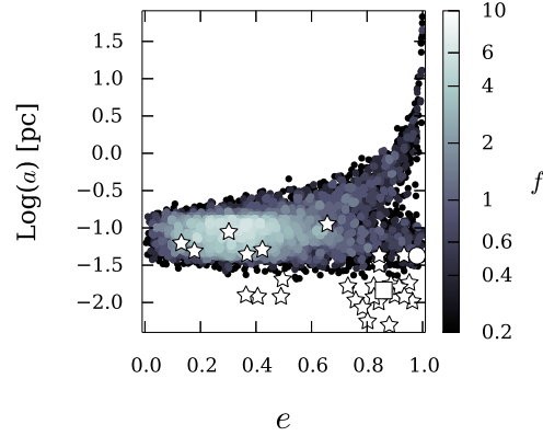
Fig. 2. Eccentricity ( e ) versus the semi-major axis ( a ) of the kicked secondary stars. The symbols mark the values of e and a for G1 (square), G2 (open circle), and for the S-cluster members (stars). The color bar represents the points density.
